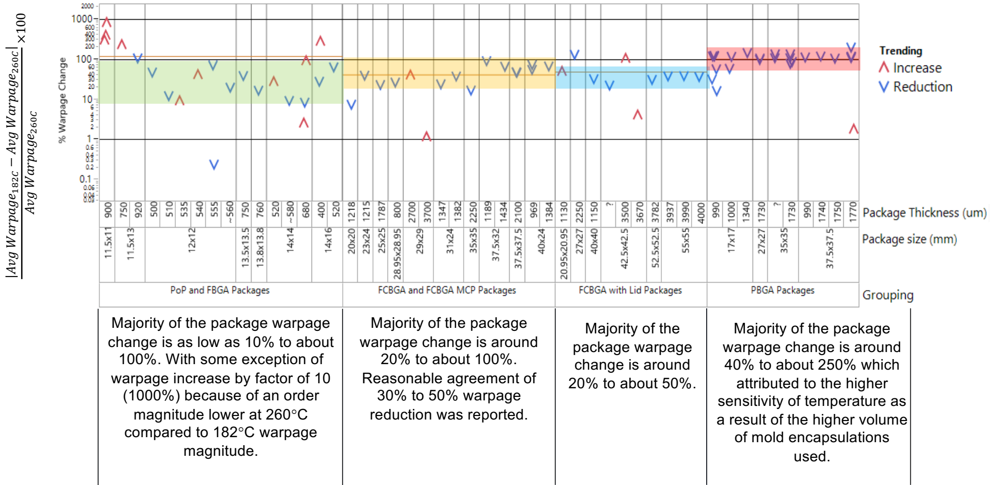
Figure 3. Package warpage change percentage as a function of different packaging technologies
