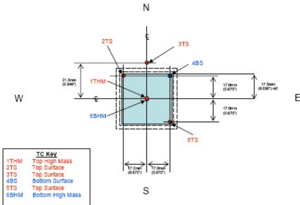
Figure 7: Rework Machine Temperature Measurement Equipment Thermocouple Locations
