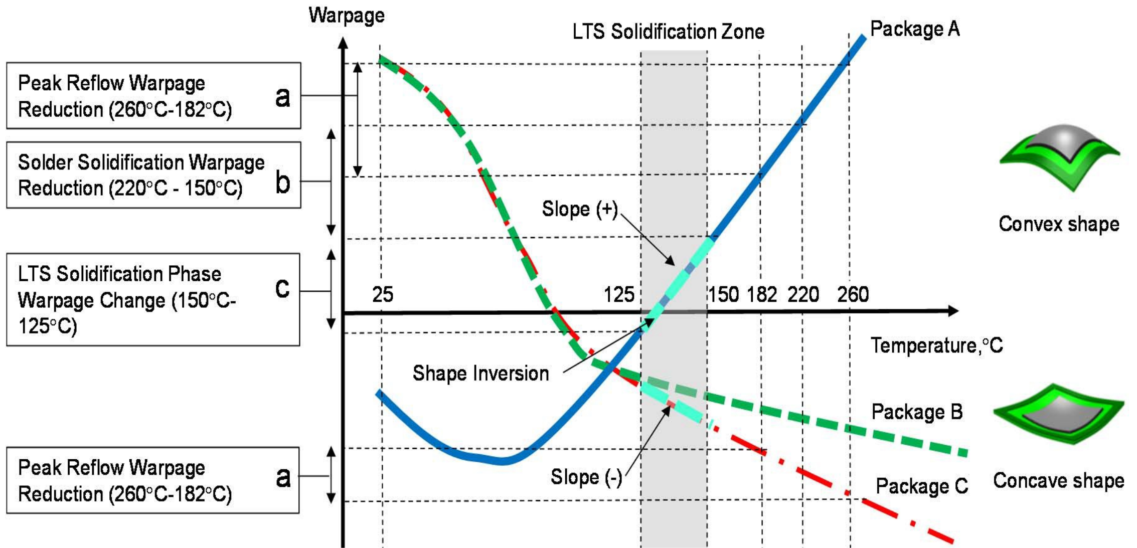
Figure 2. Typical dynamic warpage behavior and LTS key characteristics.
