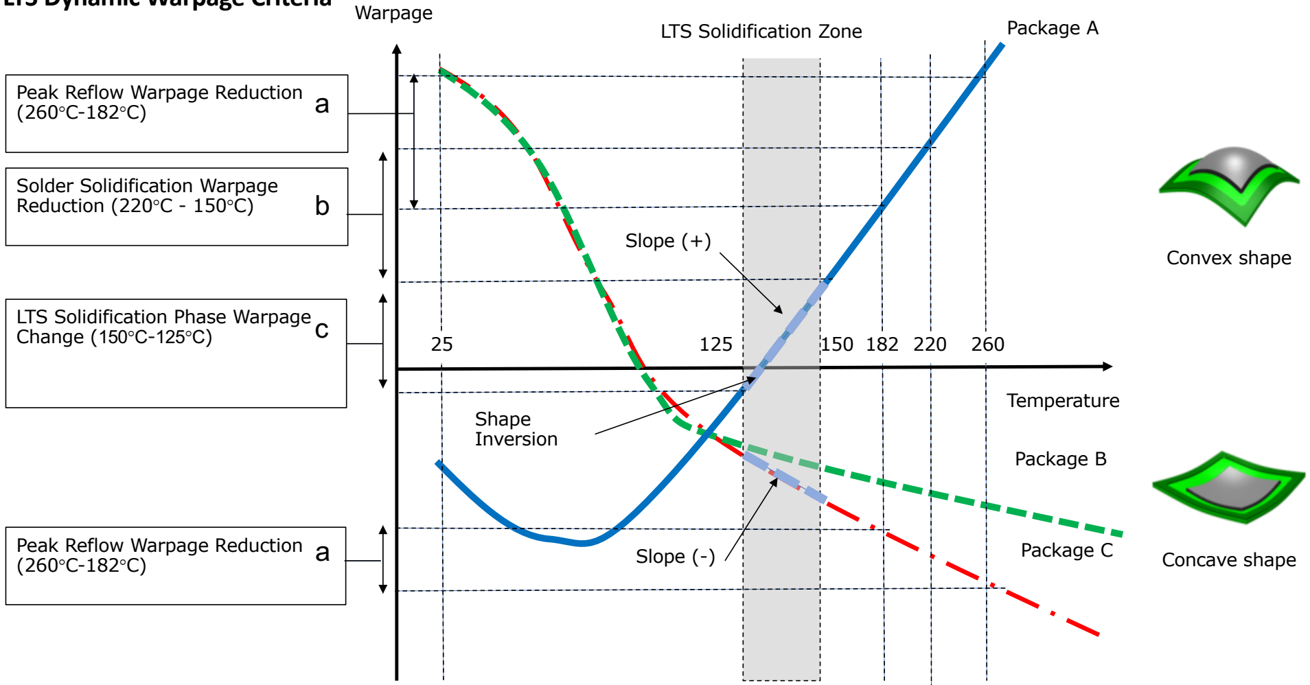
Figure 2. Dynamic warpage behavior for SAC reflow or low-temperature reflow for any package type
