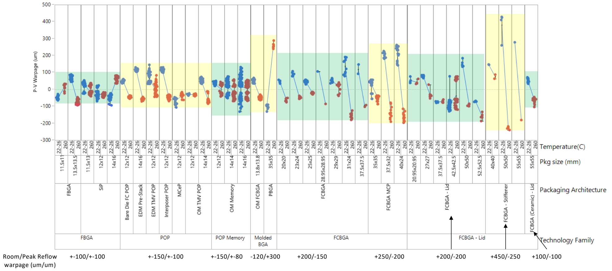
Figure 1. Typical warpage range for different packaging technology families at room and peak reflow temperatures
